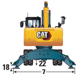
Undercarriage with 2 sets of outriggers
